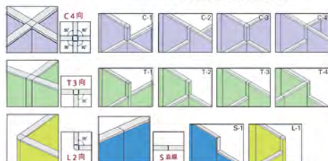
P32 Partition Unit
